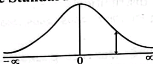
Ordinates (y) of the Standard normal curve at z
